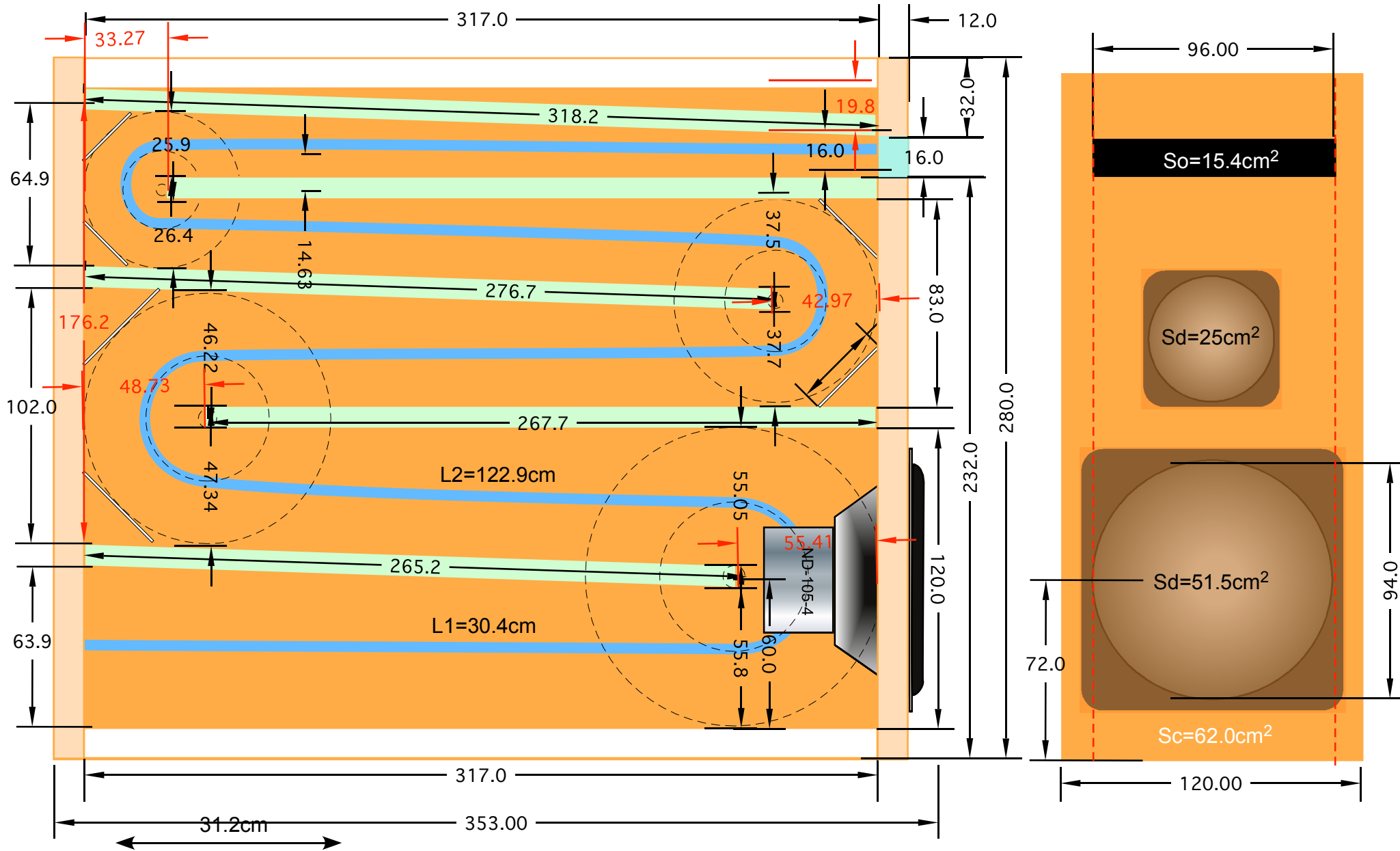
Tapered Quarter Wave Tube 4" Driver Design (17/11L)
